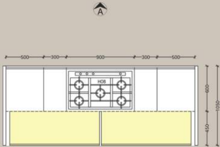
Extra Storage
