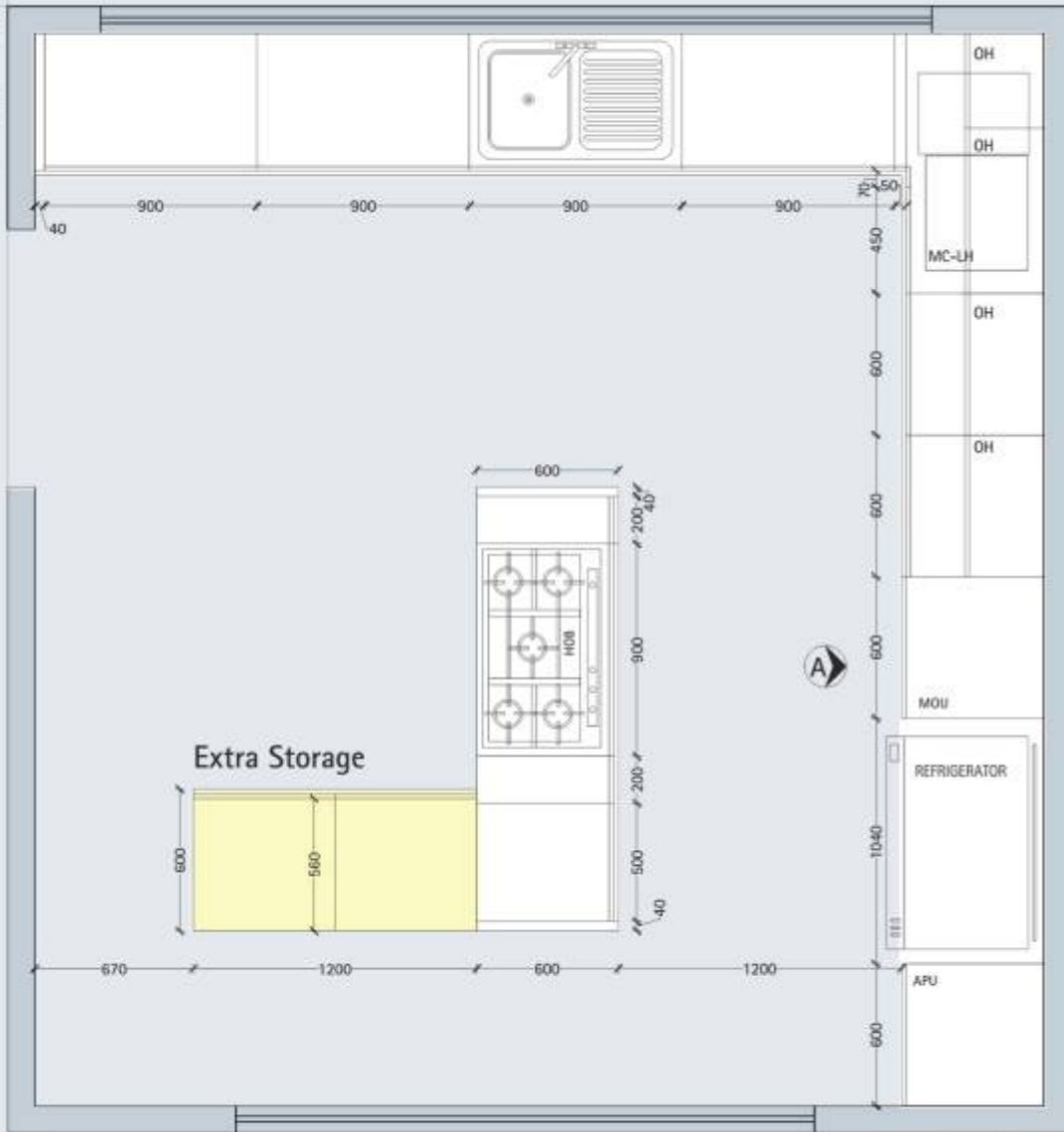
Plan
